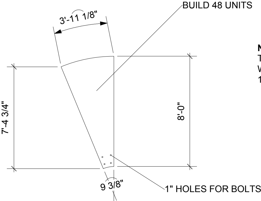
DECK DETAIL
