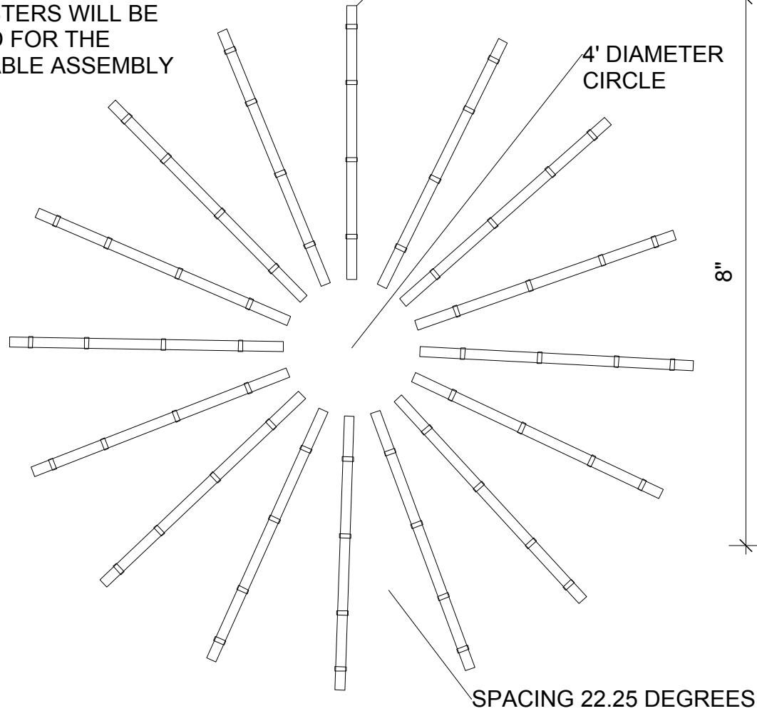
TOP VIEW SCALE: 1/4" - 1' - 0"
