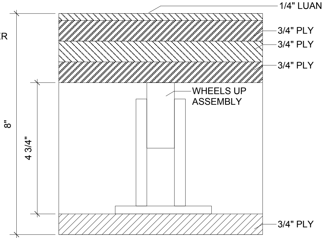
SECTION VIEW SCALE = 1:2
