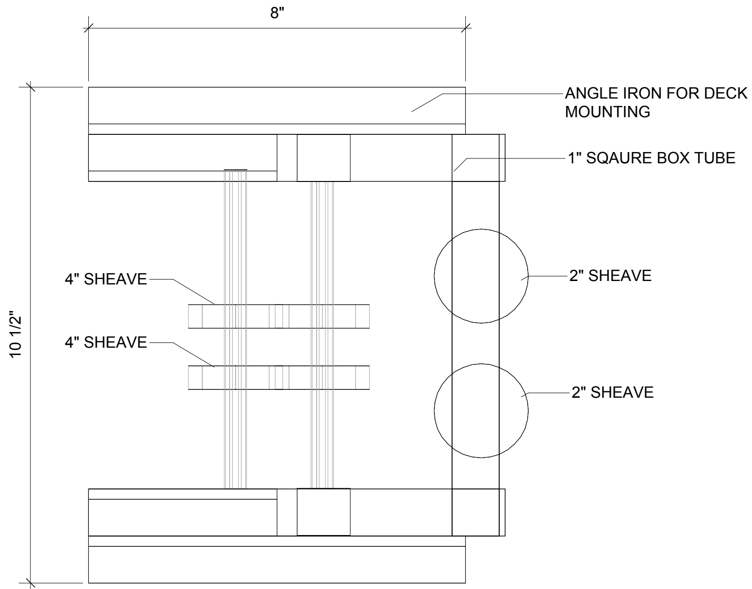
PLAN VIEW
