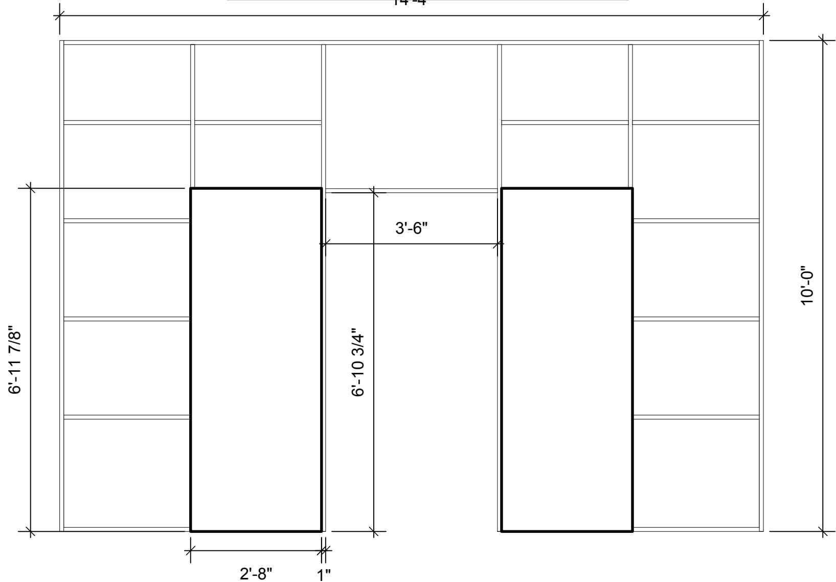
REAR VIEW WALL/POCKET DOOR
