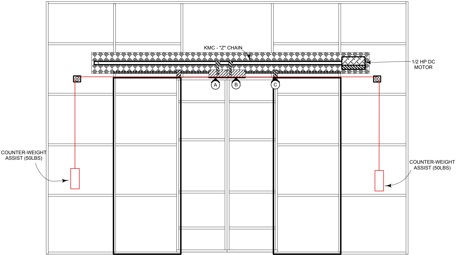
REAR VIEW OF SYSTEM
